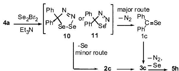
Scheme 8
